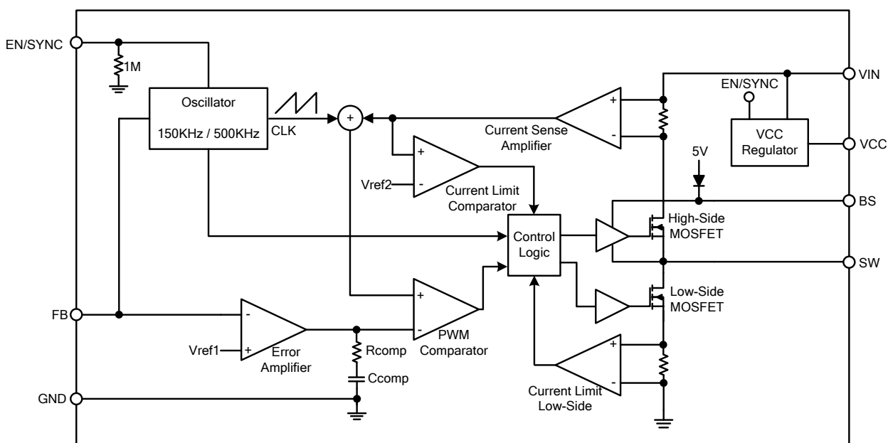
Figure 4. Block Diagram of FR9808
