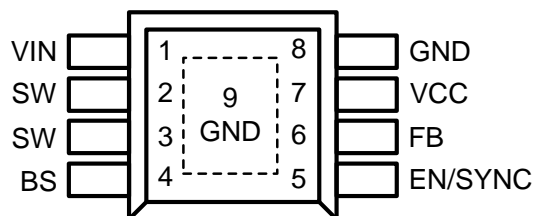
Figure 1. Pin Assignment of FR9808
