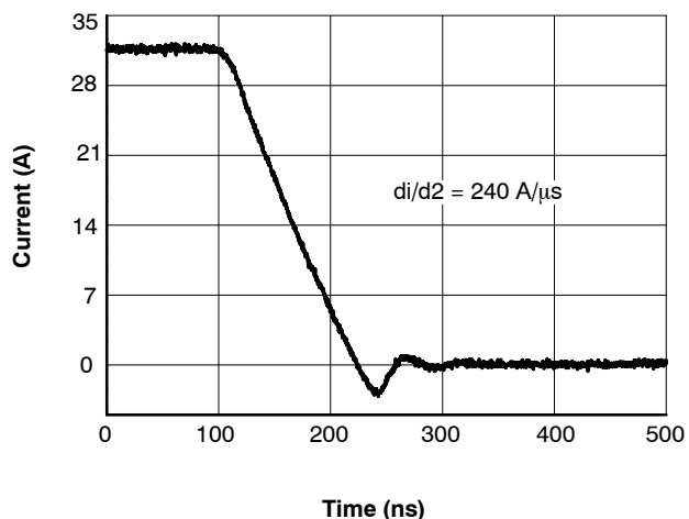
Figure 27. SyncFET Body Diode Reverse Recovery Characteristic
