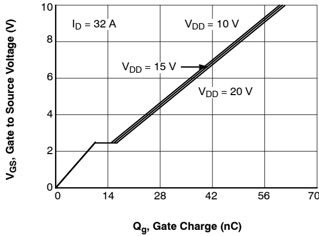
Figure 20. Gate Charge Characteristics
