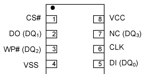
8 - LEAD VDFN
