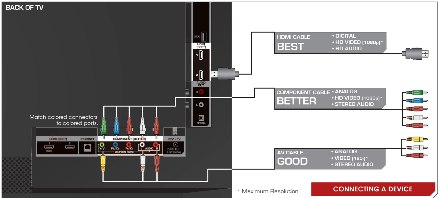
DVD/Blu-ray Player
